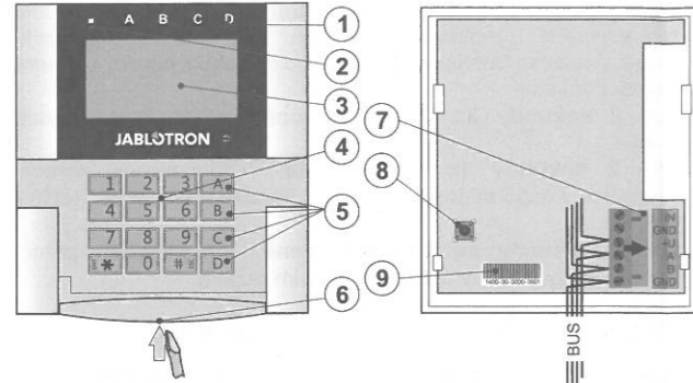
Figure 1 : 1 – status indicators; 2 – system indicator; 3 – LCD display; 4 – keypad and the RFID reader; 5 – function buttons A, B, C, D; 6 – keypad opening tab; 7 – detachable BUS terminals; 8 – tamper contact; 9 – production number
