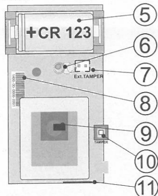
Figure 2.: 5 – battery holder; 6 – LED indicators; 7 – the JA-191PL external tamper connector; 8 – production code; 9 – PIR sensor; 10 – cover tamper contact; 11 – antenna
