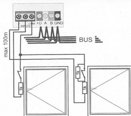
Figure 3: Loop balancing
