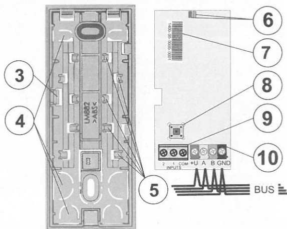
Figure 2: 3 – PCB tab; 4 – cut-out holes; 5 – fixing clips for cables coming from the top cut-out holes; 6 – red and yellow LED indicator; 7 – production code; 8 – tamper sensor; 9 – magnetic contact terminal; 10 – BUS terminal;
