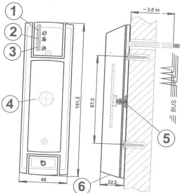
Fig: 1 – red LED indicates an armed (set) section, 2 – green LED indicates a disarmed (unset) section, 3 – yellow LED indicates fault/service mode
